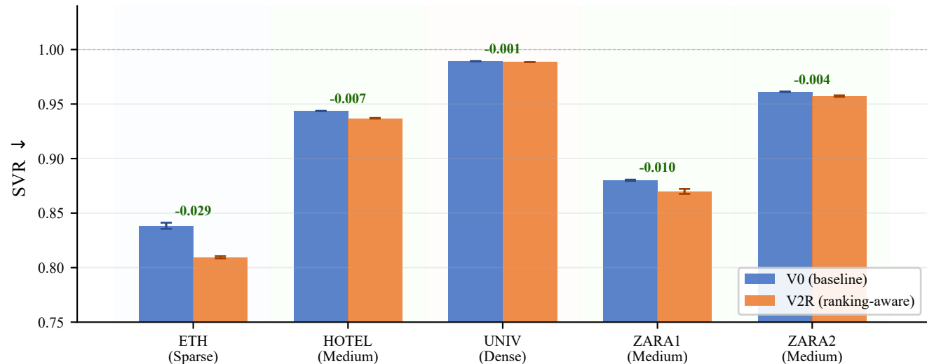
Social Violation Rate by Subset and Density Tier (3-seed mean \pm std; seeds 42, 1, 123)
